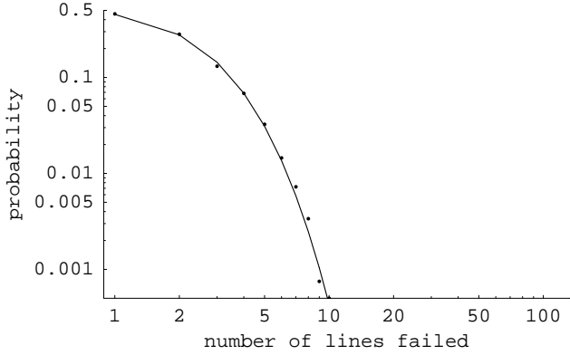
Fig. 3: IEEE 118 bus system with loading factor 0.9. Distribution of line outages estimated with branching process (solid line) compared with OPA empirical distribution (dots). Note the log-log scales.
