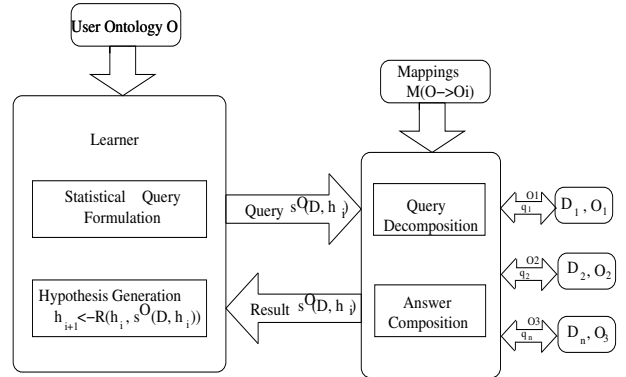
Figure 2. Learning from Distributed, Semantically Heterogeneous Data Sources [9]
