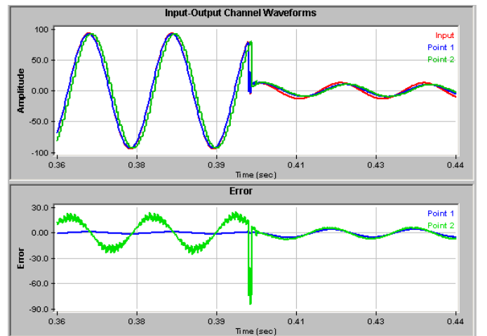
Figure 4. Snapshot of the Channel Performance One Cycle Before and After the First Fault.
