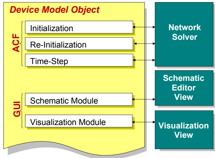
Figure 1. The Virtual Power System Architecture and Model Organization
