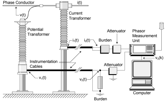
Figure 2. Typical Instrumentation Channel for DFR Data Collection
