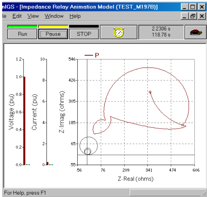
Figure 6. Animation of a Modified Impedance Relay for a Single Line to Ground Fault on the 115 kV Bus
