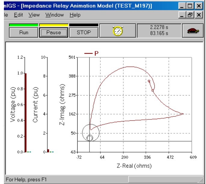
Figure 7. Animation of a Mho Relay for a Three Phase Fault on the 13.8 kV Bus
