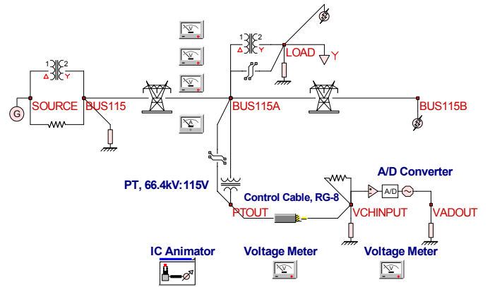
Figure 3. Example Power System for Visualization and Animation of an Instrumentation Channel
