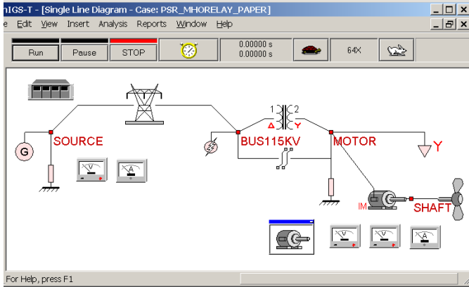
Figure 5. Example Test System For Mho Relay Animation
