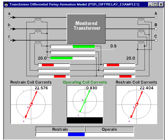
Figure 9. Animation of a Transformer Differential Relay for a Single Phase to Ground Fault on the 115 kV Bus
