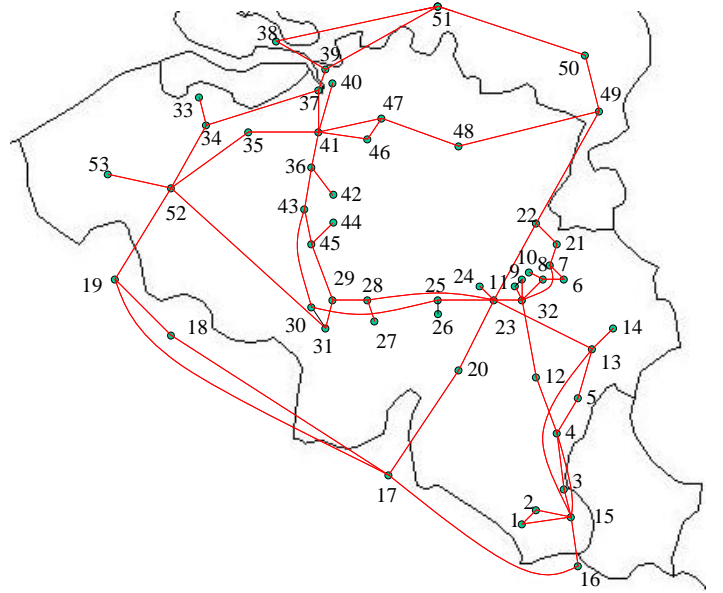
Fig. 2. Belgian high voltage network
