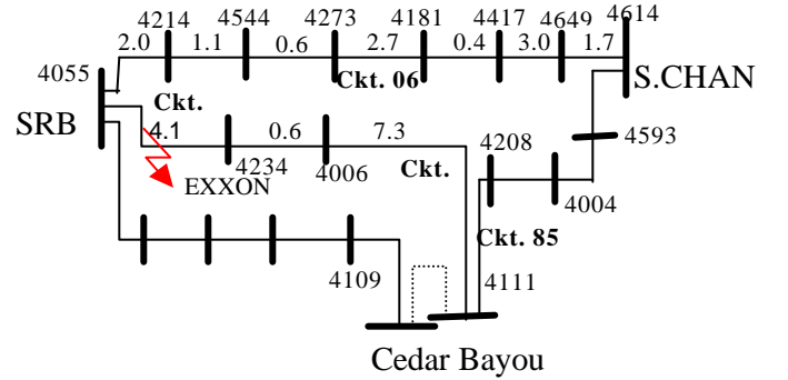
Fig. 6 One-line Diagram for case I
