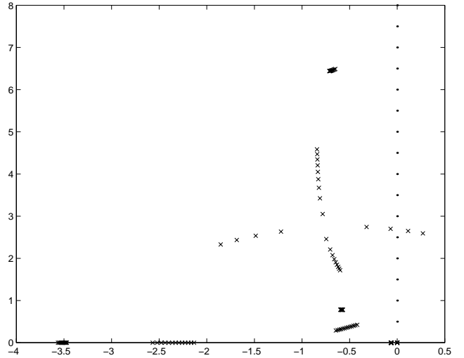
Figure 8: 9 bus eigenvalues as dispatch varies
