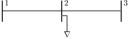
Figure 4: Three bus power system
