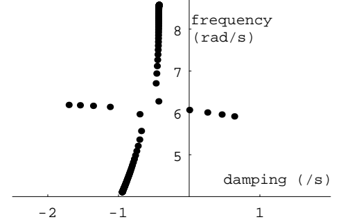
Figure 7: Eigenvalues as dispatch varies; V_{ref} = 1.11
