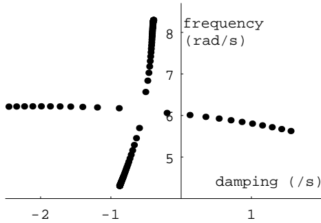
Figure 5: Eigenvalues as dispatch varies; V_{ref} = 1.07
