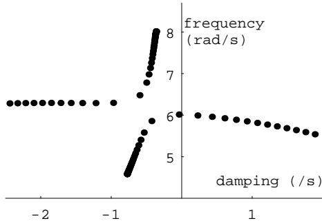
Figure 6: Eigenvalues as dispatch varies; V_{ref} = 1.03
