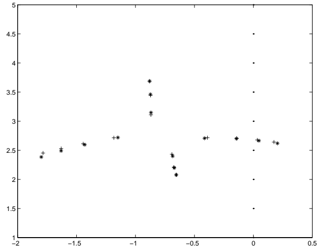
Figure 11: Predicting eigenvalue movement near resonance; + = predicted eigenvalues, * = actual eigenvalues.
