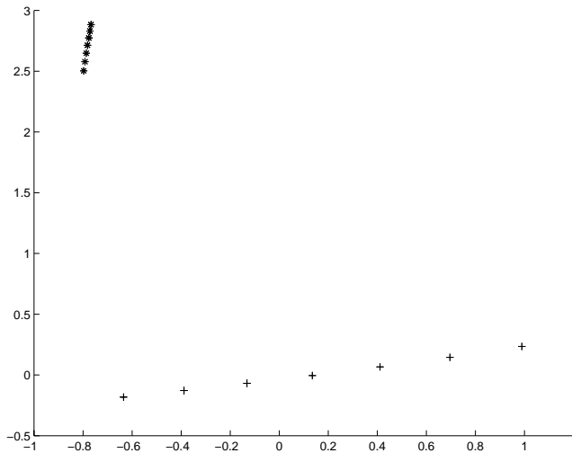
Figure 10: Variation in \lambda and \mu near strong resonance; * = \lambda , + = \mu .
