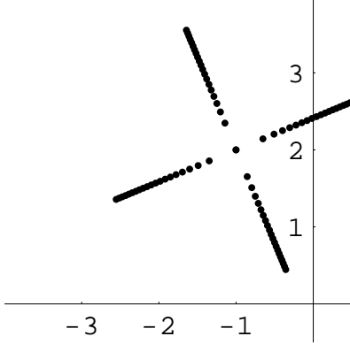
Figure 1: Two modes of matrix M_1 encountering strong resonance real number \alpha :
