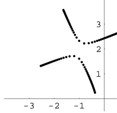
Figure 2: Two modes of matrix M_2 moving near strong resonance
