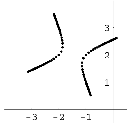
Figure 3: Two modes of matrix M_3 moving near strong resonance
