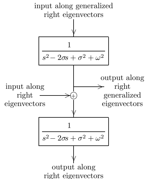
Figure 9: Modes at strong resonance
