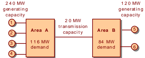
Figure 4 Transmission Network Block Diagram
