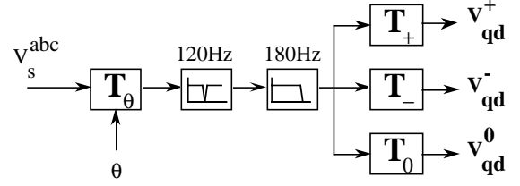
Figure A1. Synchronous frame sequence component transform block diagram
