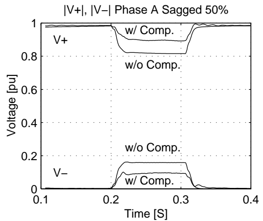
Figure 8. Magnitude of positive and negative sequence components during single line to ground fault with and without StatCom.
