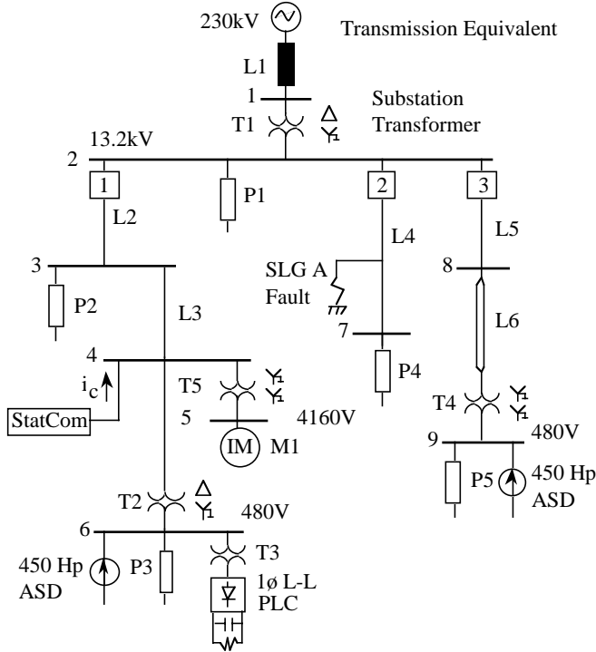
Figure 6. Distribution system model for simulations.
