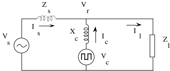
Figure 2. Reduced model for regulator circuit.
