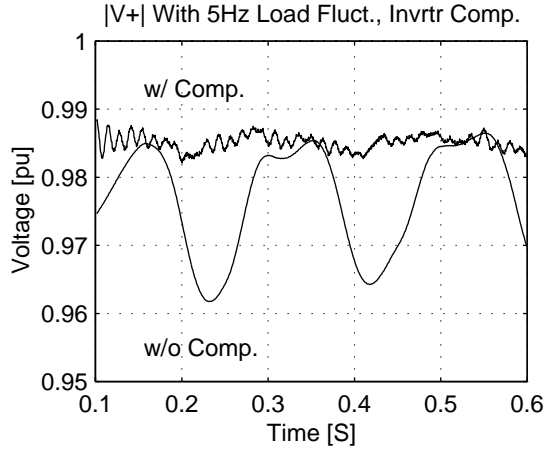
Figure 9. Three phase voltage during 5Hz load variation with and without StatCom.
