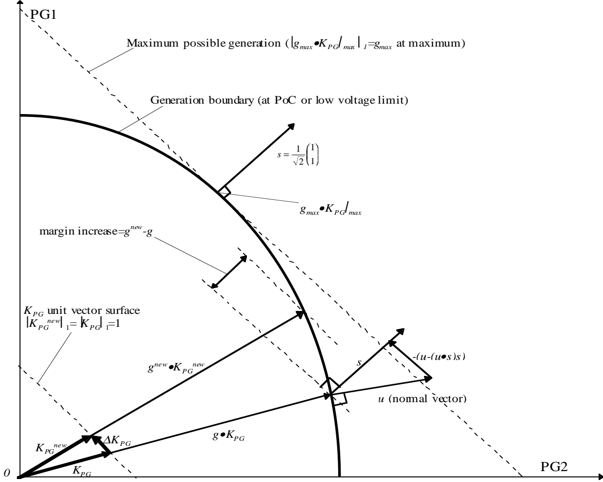
Fig. 1: The search algorithm.
