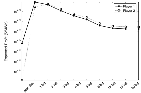
(b) Expected profit with demand independent of the past. Player 1 has a higher repair rate.
