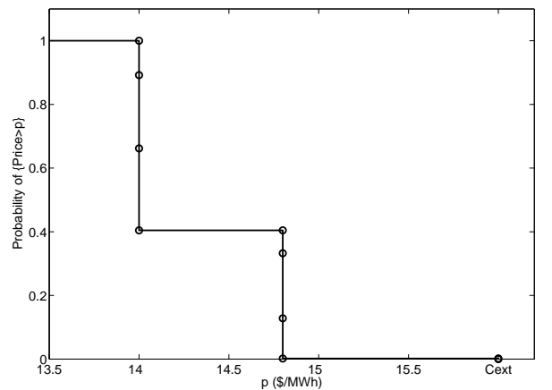
Fig. 2. EPDC from the PGM method with the price competition model.
